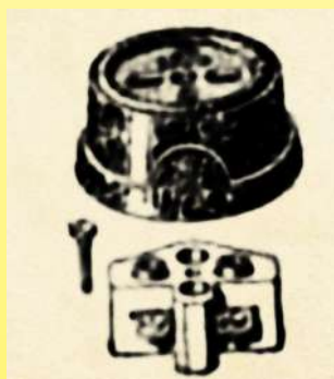
Power socket with porcelain base and bakelite lid (1932 Maure Catalog, Ultimheat Museum)
